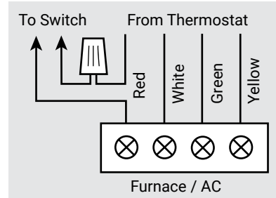
Switch Wiring Instructions for 3/4" CS-1 Float Switch (A)
